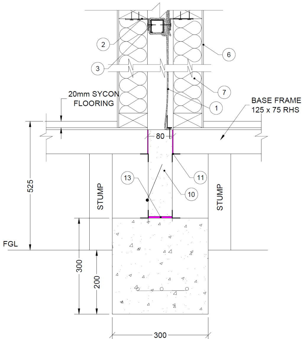
Figure 3 – Optional Wall Base Detail
