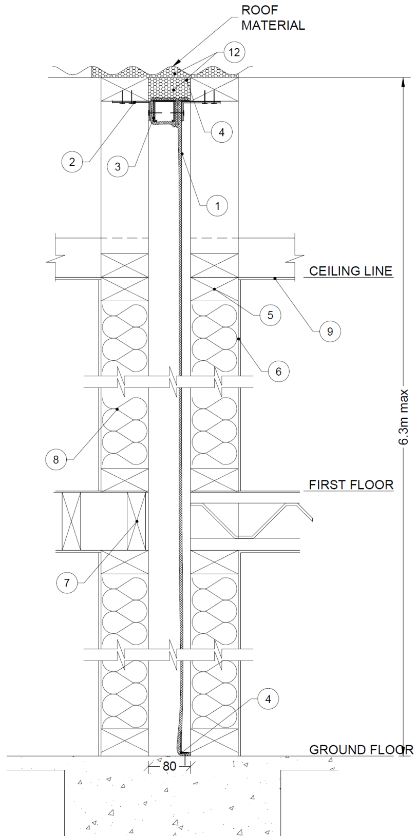
Figure 2 – Section Elevation of Party Wall with TBA Firefly Titan Central Barrier
