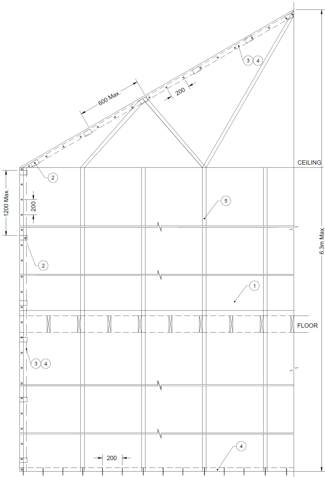
Figure 1 –Elevation of Party Wall System with TBA Firefly Titan Central Barrier
